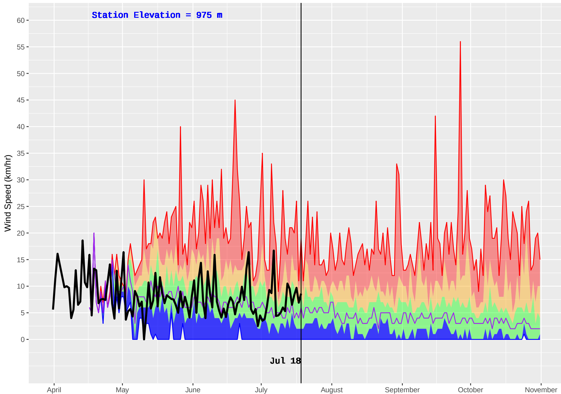
MCGREGOR 2 (192) : Historical (1986–2016) and Current (2018) Daily Wind Speed
