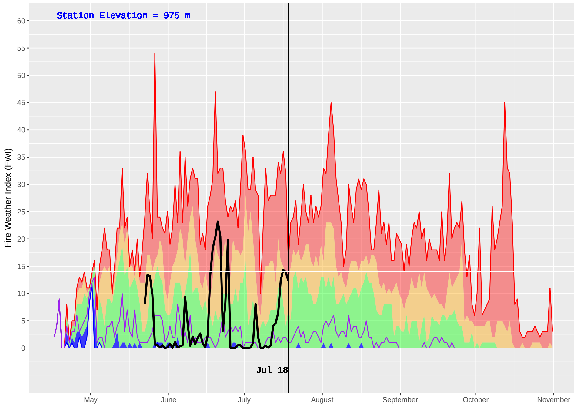
MCGREGOR 2 (192) : Historical (1986–2016) and Current (2018) Daily Fire Weather Index (FWI)
