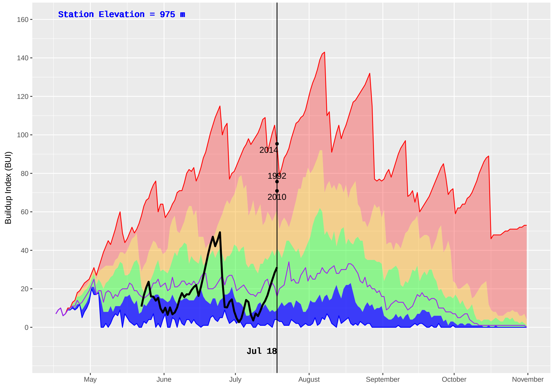
MCGREGOR 2 (192) : Historical (1986–2016) and Current (2018) Daily Buildup Index (BUI)
