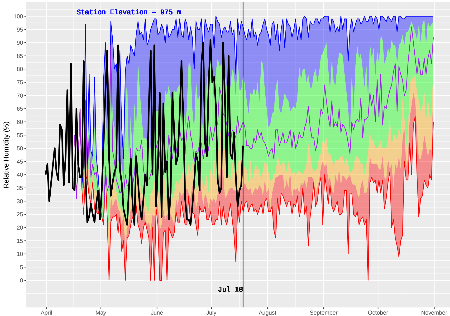
MCGREGOR 2 (192) : Historical (1986–2016) and Current (2018) Daily Relative Humidity
