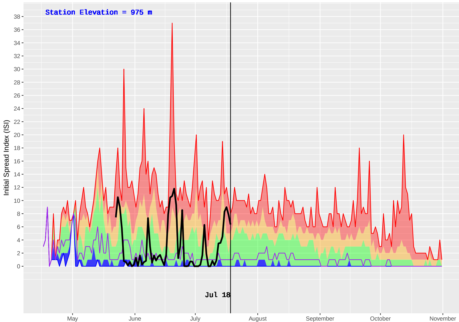
MCGREGOR 2 (192) : Historical (1986–2016) and Current (2018) Daily Initial Spread Index (ISI)
